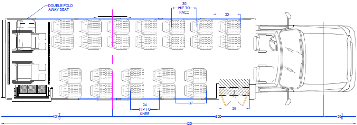
KSIR Super Pro F-550 Cutaway - Model F5G-350 24 Passengers & 2 W/C or 26 Passengers & 1 W/C
