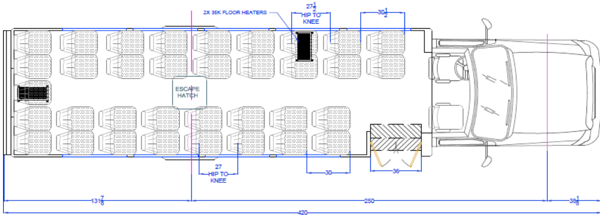
Super Pro F-550 Model 350 29 Passengers with 32" Rear Luggage
