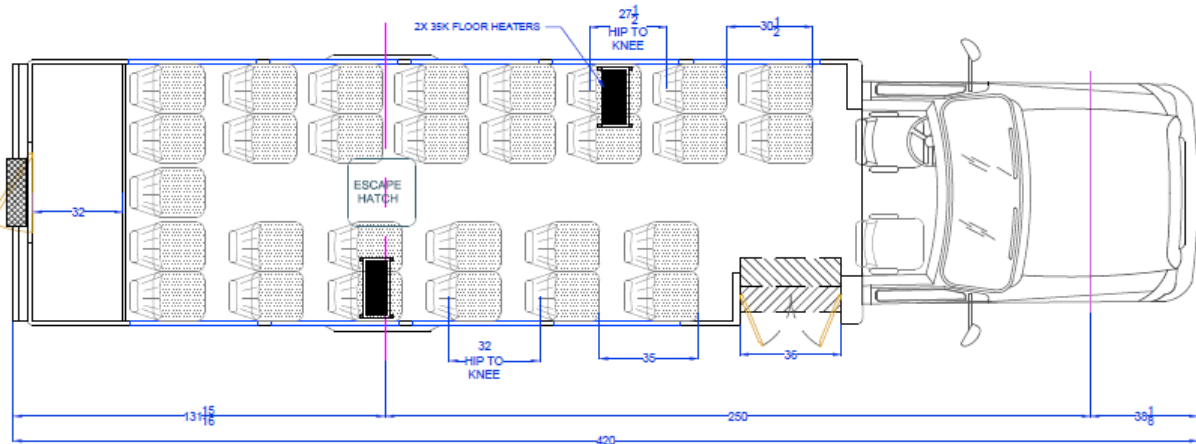
KSIR Super Pro F-550 Cutaway - Model F5G-350 24 Passengers & 2 W/C or 26 Passengers & 1 W/C
